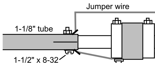
Figure-13: Resonator Installation Detail
