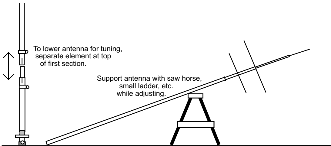
Figure-16: Handling antenna for tuning operation
